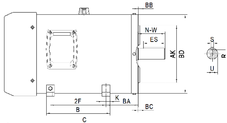
Frame 250T-280T
